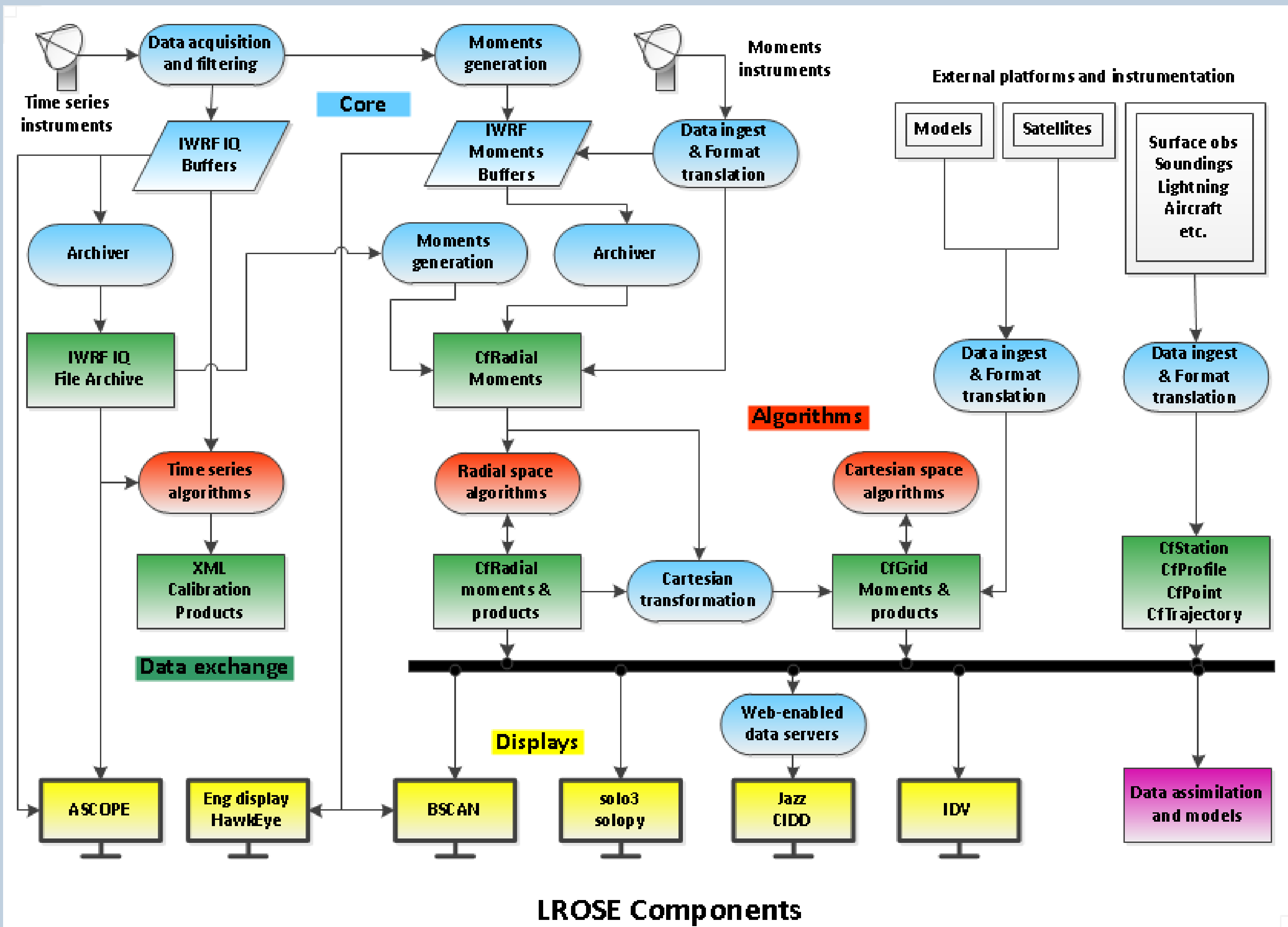
LROSE Components
