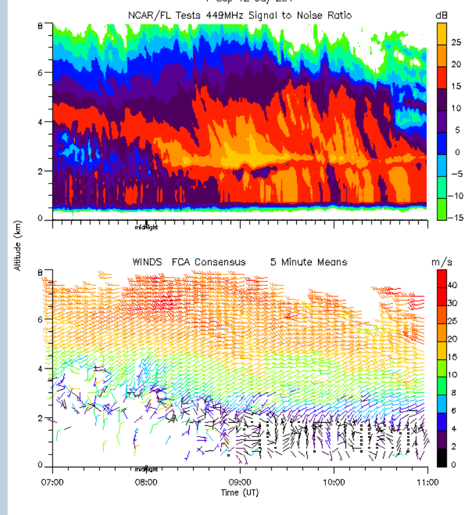
XPROF profiler display, Boulder FootHills lab 2012/09/07
