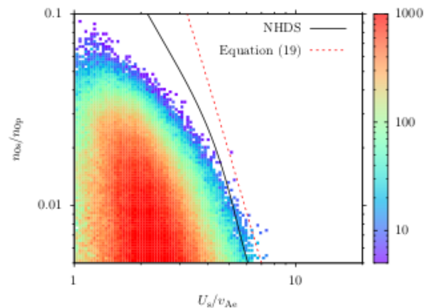
Figure 6. Data distribution of the analyzed solar-wind interval in the n_{0s}/n_{0p} vs. U_s/v_{Ae} plane. The color-coding shows the probability density in the corresponding bin in arbitrary units. The black line shows the isocontour of maximum growth rate \gamma_m = 10^{-3}|\Omega_e| for the oblique FM/W instability from our NHDS solutions. The red dashed line shows Equation (19) for \theta = 60^\circ , and w_c = v_{Ae} = w_s .
