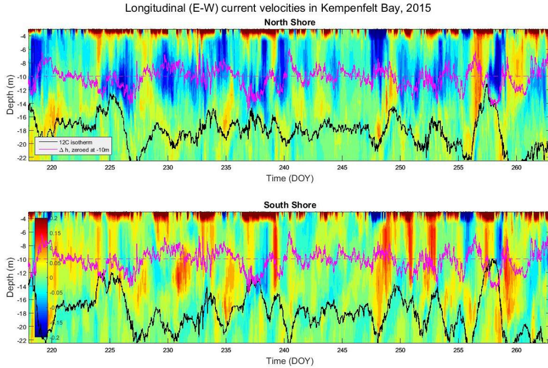
Figure 4: Current velocity profile in Kempenfelt Bay. Positive (red) is easterly; negative (blue) is westerly. 12°C isotherm is superimposed in black. Magenta line is the tilt of the thermocline ( dh/dy ) across Kempenfelt Bay, zeroed at -10 m. Positive values ( > -10 m) indicate a tilt from north to south.
