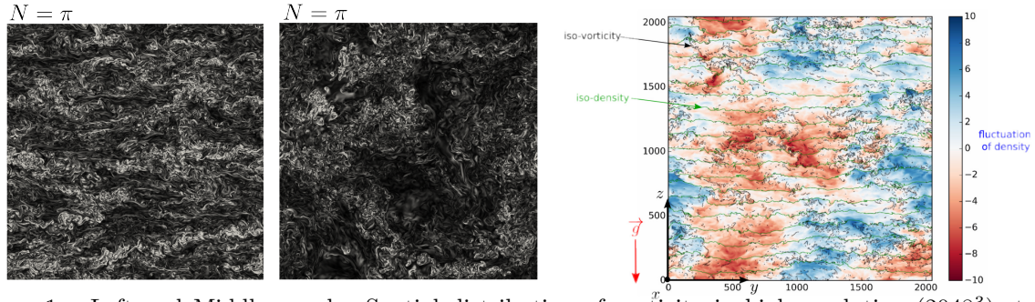
Figure 1: Left and Middle panels: Spatial distribution of vorticity in high resolution ( 2048^3 ) stably stratified turbulence DNS. N = \pi is the Brunt-Väisälä frequency, here corresponding to moderately small Froude number of order 0.1. Left : horizontal plane cut; Middle : vertical plane cut. One clearly observes both strong horizontal motion and vertical layering, as well as large-scale anisotropy and small-scale more isotropic “worms”, corresponding to the difference of energy among scales and orientations presented in Fig. 3 spectra. Right panel : Visualization of the 2048^3 DNS field in a vertical plane of strongly stratified turbulence: isodensity fluctuations are shown in color. Isovorticity lines are shown in black, and isolines of total density in blue.
