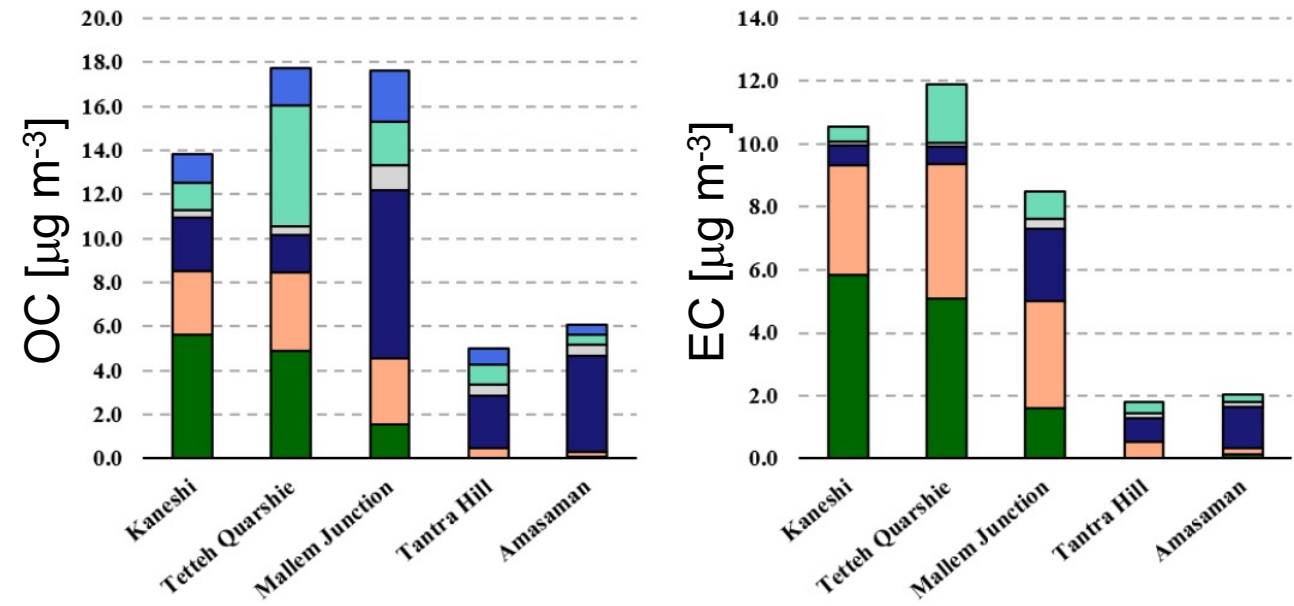
Sources of EC and OC at roadside sites across Accra, Ghana
